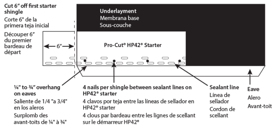
DIAGRAM 1 STARTER COURSE
