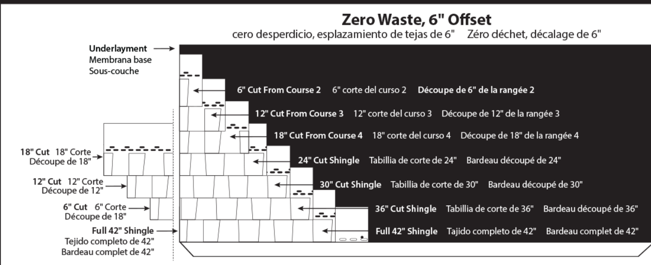
DIAGRAM 3 SHINGLE OFFSET
